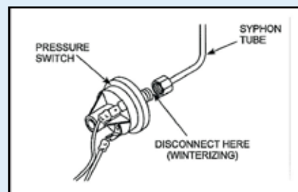
PRESSURE SWITCH
